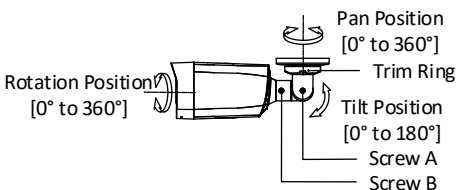
Figure 2-2 3-Axis Adjustment
