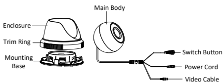
Figure 1-4 Overview of Type II Camera
