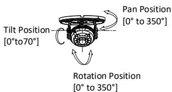
Figure 2-14 3-Axis Adjustment
