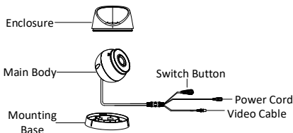
Figure 1-6 Overview of Type III Camera
