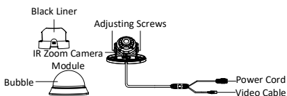
Figure 1-9 Overview of Type VI Camera
