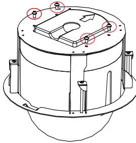
Figure 2-6 Remove 4 screws
