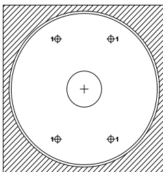
Figure 2-19 Drill Template
