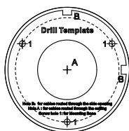
Figure 2-4 Drill Template
