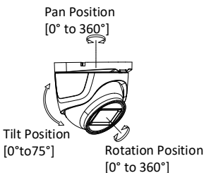
Figure 2-10 3-axis Adjustment
