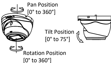
Figure 2-11 3-axis Adjustment
