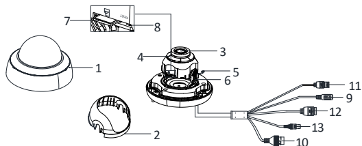
Figure 1-2 Overview of Type II Camera
