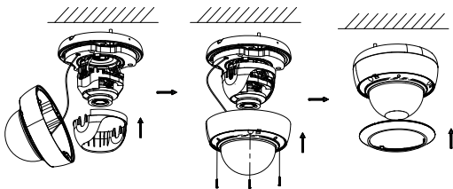
Figure 2-5 Secure Black Liner and Bubble
