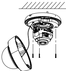
Figure 2-4 Secure the Camera
