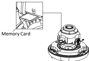
Figure 2-2 Install the Memory Card
