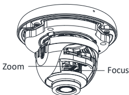
Figure 2-8 Zoom/Focus Lever
