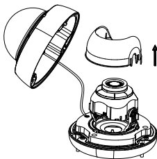
Figure 2-1 Remove the Bubble and Black Liner
