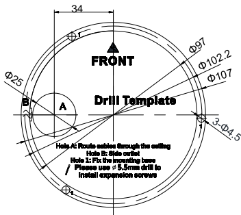
Figure 2-3 The Drill Template
