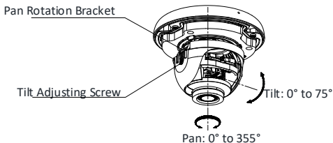
Figure 2-7 Angle Adjustment
