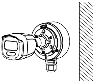
Figure 2-7 Combine the Junction Box Cover back to its Body 8. Repeat the step 5 to 6 of 2.1.1 Ceiling/Wall Mounting without Junction Box to finish the installation.
