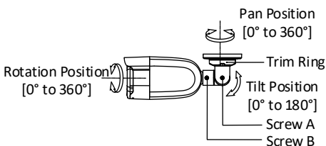
Figure 2-10 3-Axis Adjustment
