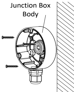
Figure 2-6 Secure the Junction Box on the Wall/Ceiling 6. Route the cables through the bottom cable hole, or the side cable hole of the junction box. 7. Combine the junction box cover with its body.
