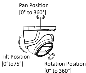
Figure 2-15 3-axis Adjustment
