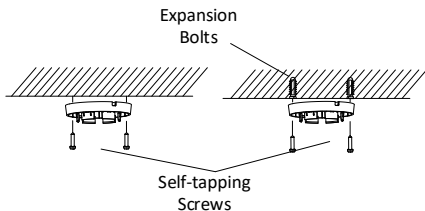
Figure 2-8 Fix the Mounting Base to the Ceiling
